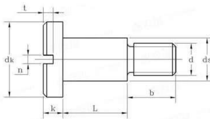
Dimensions of Metric DIN 923 Slotted Pan Head Screws with Shoulder
