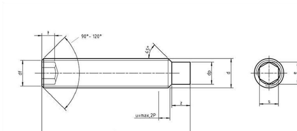
Dimensions of Metric DIN 915 hexagon socket set screws with dog point
