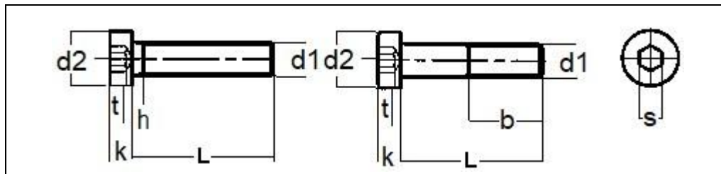
Dimensions of Metric DIN 7984 Low Head Hexagon Socket Cap Screws
