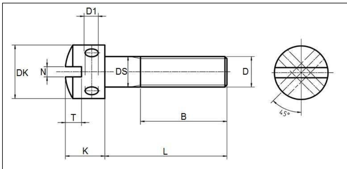
Dimensions of DIN 404 Slotted Capstan Screws
