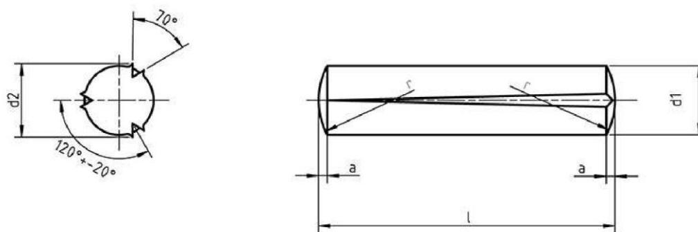
Dimensions of Metric DIN 1472 Grooved Pins, Half Length Taper Groove
